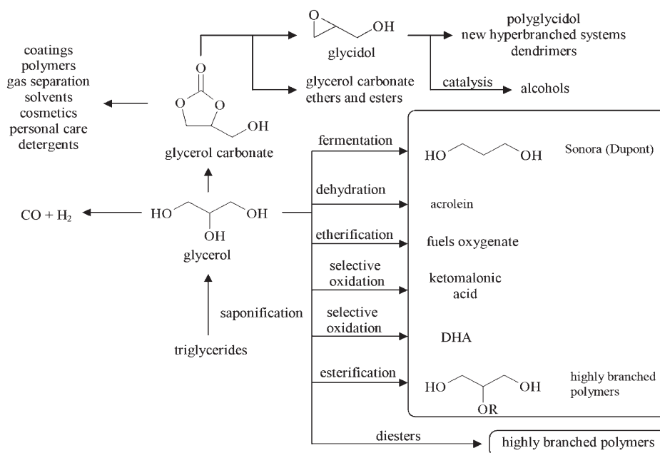
Scheme 2. Glycerol as a platform for functional chemicals (see text for details).
