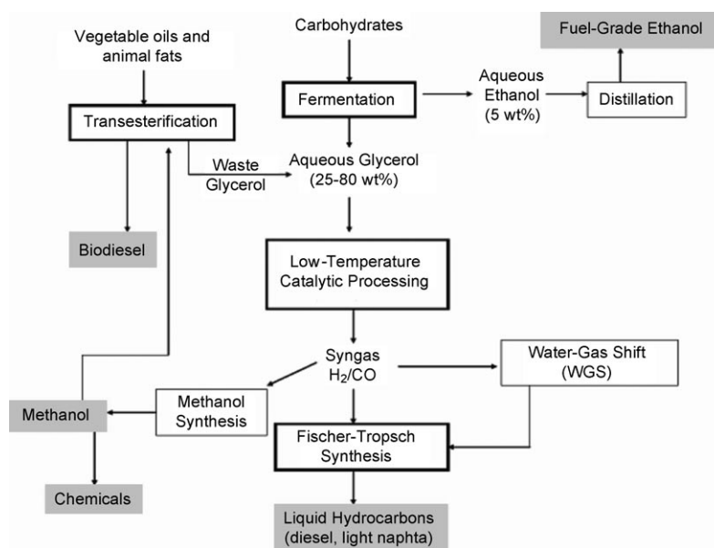
Scheme 4. Schematic view of liquid fuel and chemical production through catalytic processing of glycerol (reproduced from Ref. [29], with permission).
