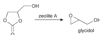
Scheme 6. Glycidol forms easily from glycerol carbonate, catalyzed by zeolite A (or \gamma -alumina) under reduced pressure.
