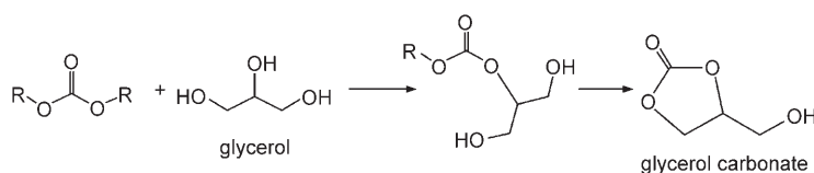
Scheme 5. Glycerol carbonate may be formed from the reaction of a dialkyl carbonate with glycerol, with an intermediate that undergoes a second esterification.
